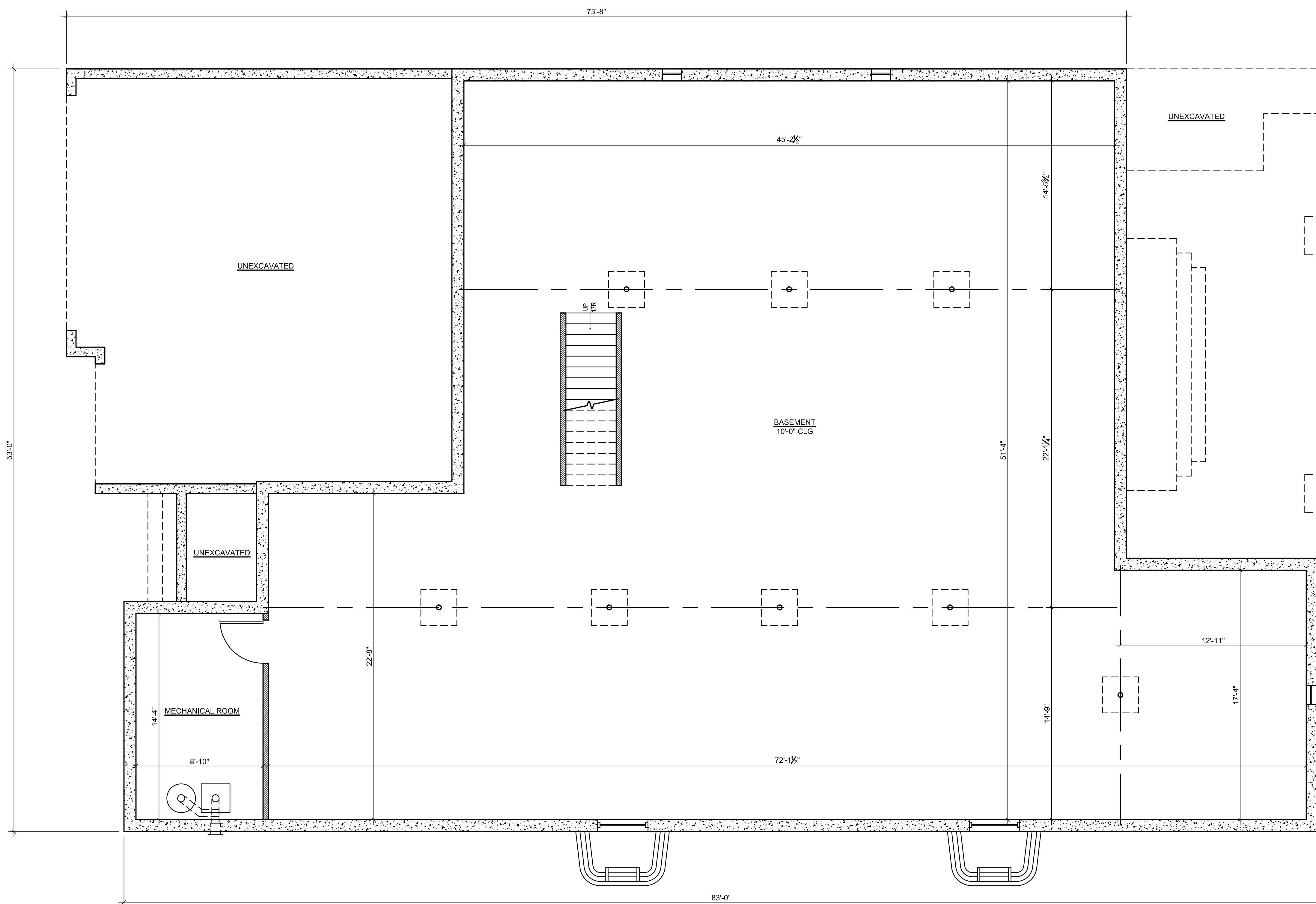
BASEMENT PLAN SCALE: 1/4" = 1'-0"
