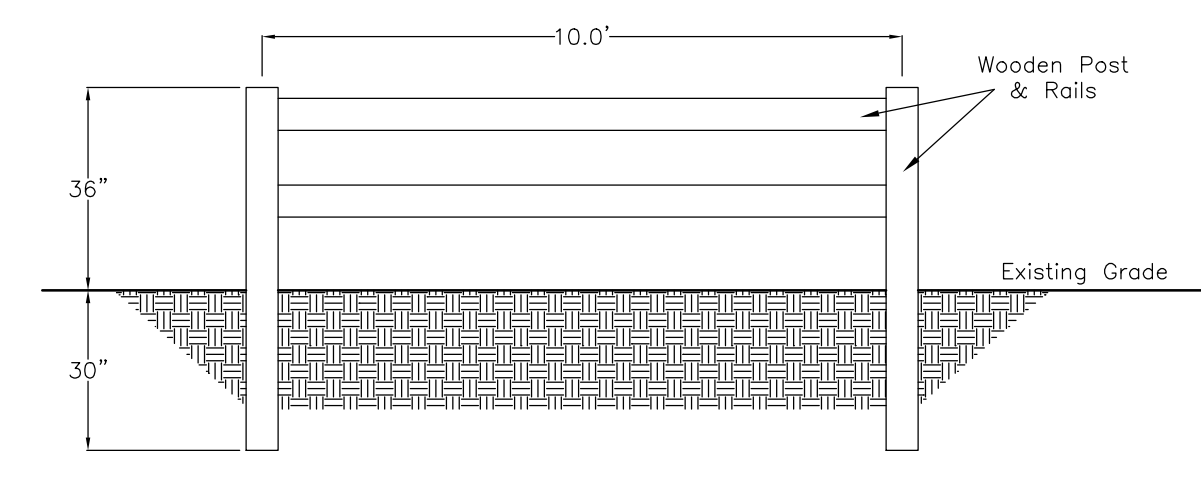
POST & RAIL FENCE DETAIL SCALE: NOT TO SCALE
